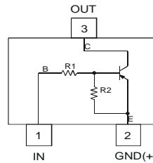
Schematic and Pin Configuration
